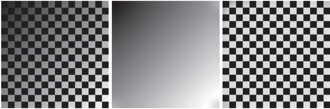
FIGURE 3.42 (a) Image shaded by a shading pattern oriented in the -45^\circ direction. (b) Estimate of the shading patterns obtained using lowpass filtering. (c) Result of dividing (a) by (b). (See Section 9.8 for a morphological approach to shading correction).
